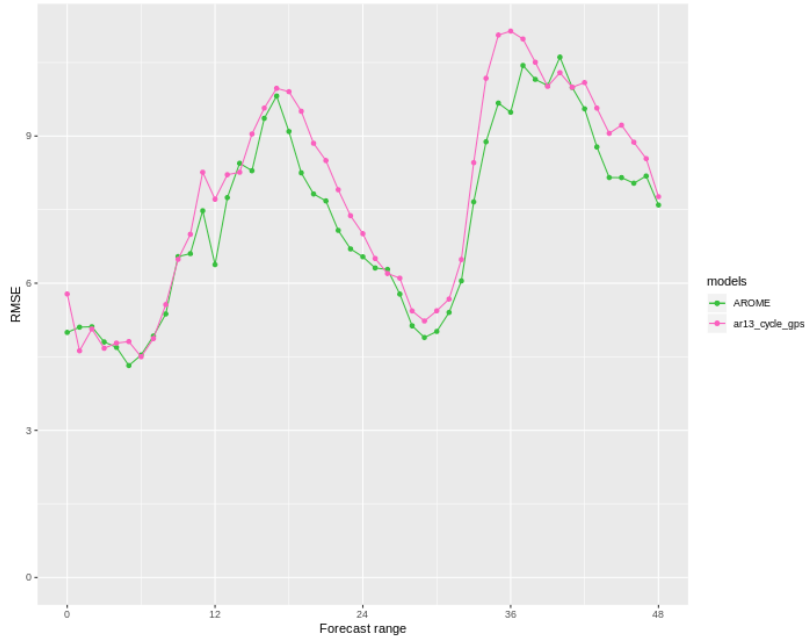
H2m RMSE 00h Runtime
