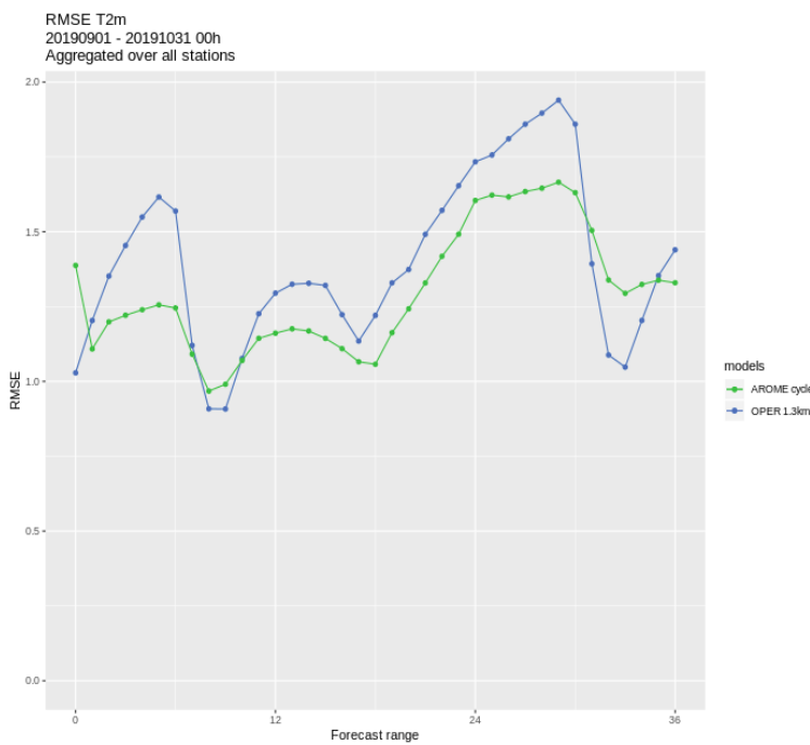
T2m RMSE 00h Runtime
