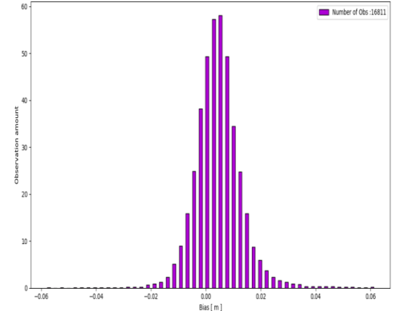
Error density distribution for all observations used from 01-01-2020 to 31-01-2020
