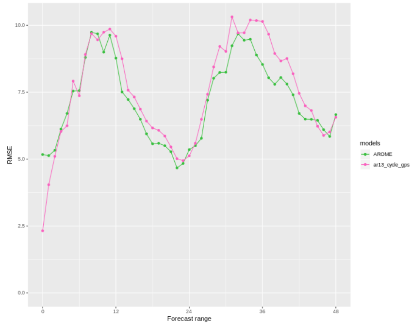
H2m RMSE 12h Runtime
